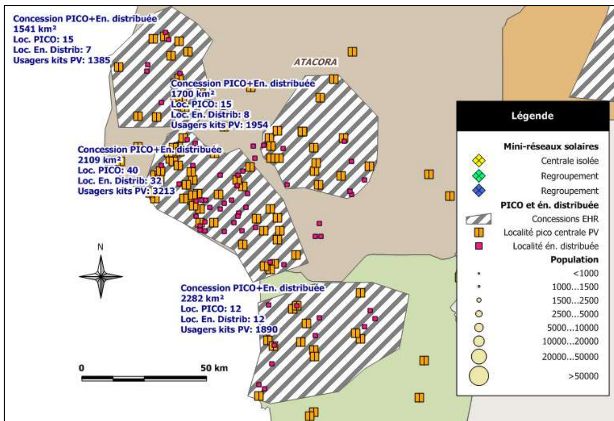
Figure 56: Concessions SSD - ATACORA et nord DONGA
